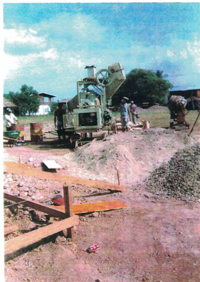
Mixing concrete with concrete mobile and column placement, Baker Leader VI, Laos
